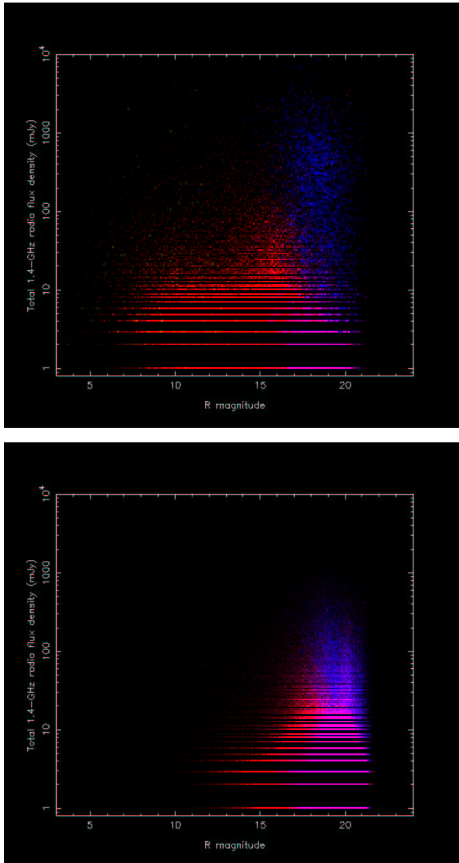
Fig. A.8. 1.4-GHz total flux density, including lobes where detected, from FIRST and NVSS, against R magnitude for (top) the previously identified sources and (bottom) the newly identified sources in the catalogue. Colours as for Fig. A.6. The top figure contains 52,995 data points, the bottom one 274,505. Quasars are over-represented for visibility.
